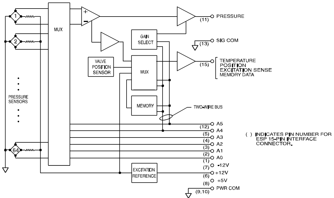
Figure 4.1 Block Diagram of a DTC Scanner
