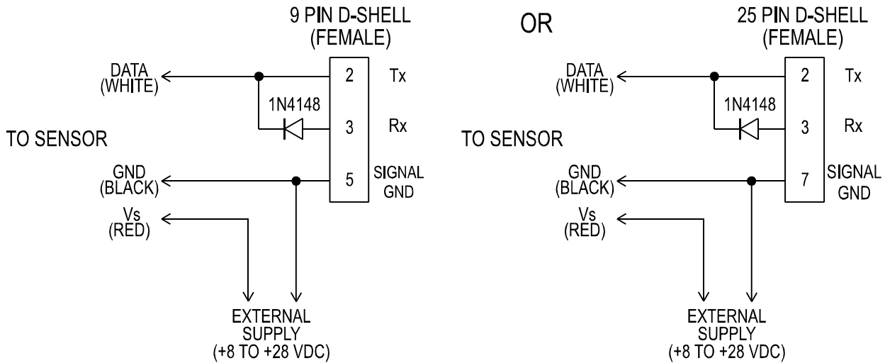
Sensor Connections to 9-Pin or 25-Pin D-Shell RS-232 Serial Port
